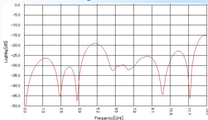
Return Loss: 2xThrough
